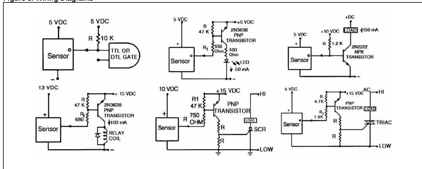
Figure 3. Wiring Diagrams
